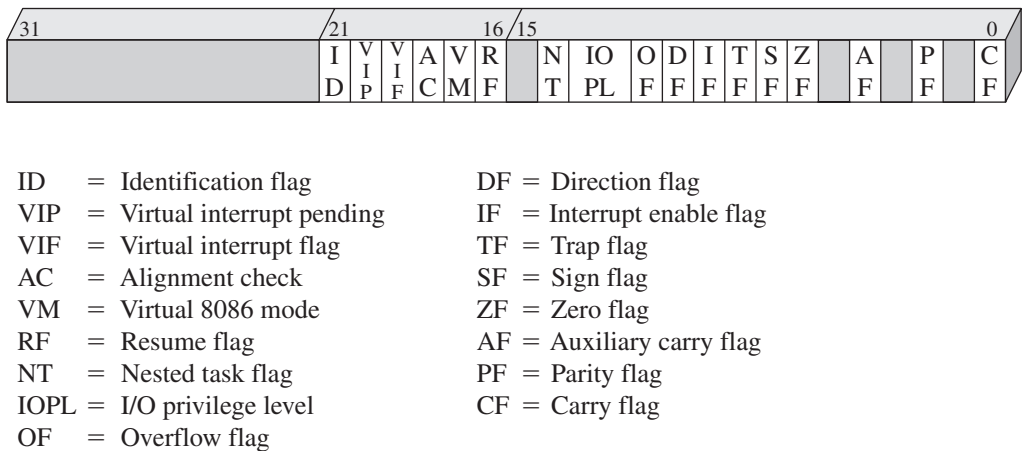
Figure 3.12 Pentium II EFLAGS Register
